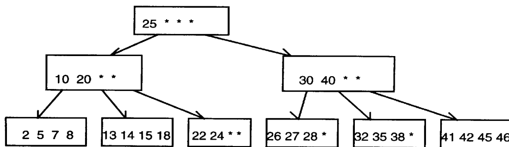
Figure 2 – B-tree of order 2 Figure 2 – Arbre de type B d'ordre 2
