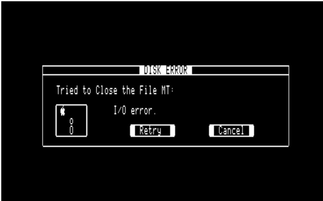
Figure 3. A text-mode message box constructed with MouseText characters.
